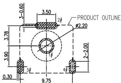
RECOMMENDED PCB LAYOUT TOP VIEW TOLERANCE:±0.05
