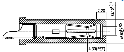
MATING PLUG DP550200-0129-60000H
