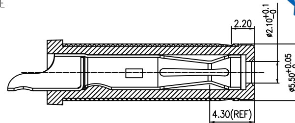
MATING PLUG
