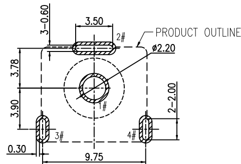
RECOMMENDED PCB LAYOUT TOP VIEW TOLERANCE:±0.05
