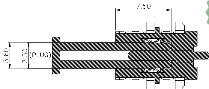
MATING PLUG SECTION
