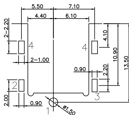
RECOMMENDED PCB LAYOUT TOP VIEW TOLERANCE±0.05mm
