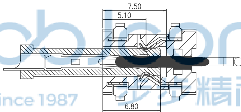
DC JACK INSERT DEPTH
