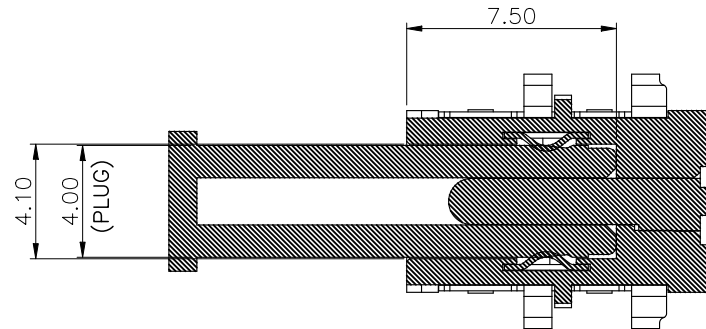
MATING PLUG SECTION
