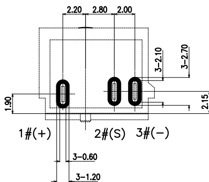
PCB LAYOUT (TOP VIEW) TOLERANCE: \pm 0.05
