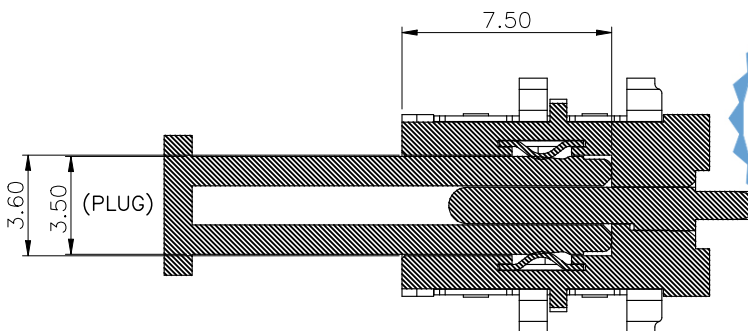
MATING PLUG SECTION
