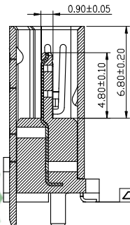
SECTION-B-B
