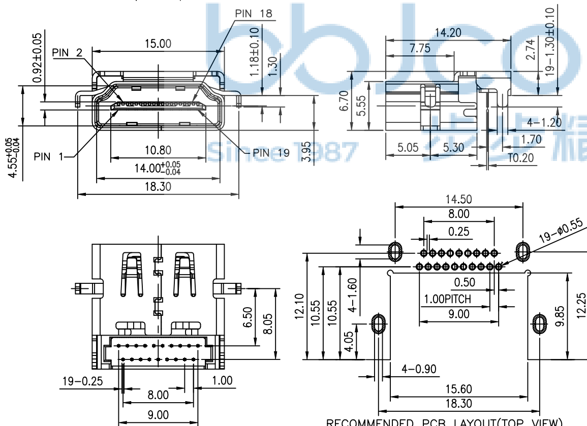
RECOMMENDED PCB LAYOUT(TOP VIEW) (THICKNESS=1.0±0.10mm) (TOLERANCE=±0.05mm)
