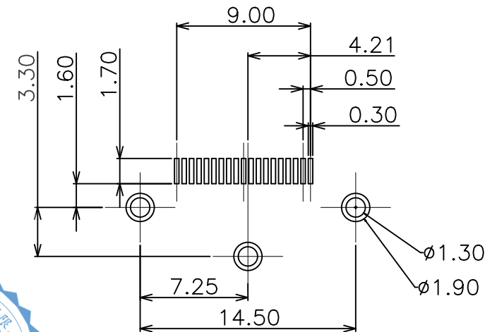
PCB LAYOUT(TOP VIEW) (T=1.60mm)
